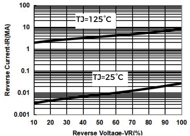
Fig.2-Typical Reverse Characteristics
