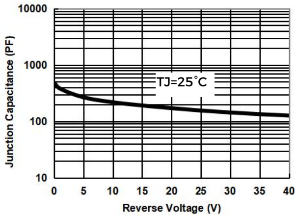
Fig.1-Typical Junction Capacitance
