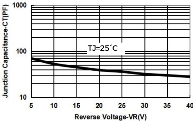
Fig.1-Typical Junction Capacitance
