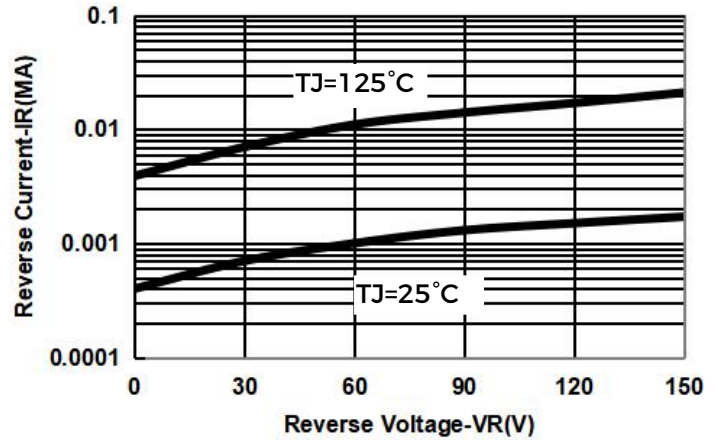
Fig.2-Typical Reverse Characteristics
