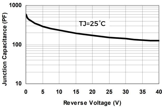
Fig.1-Typical Junction Capacitance
